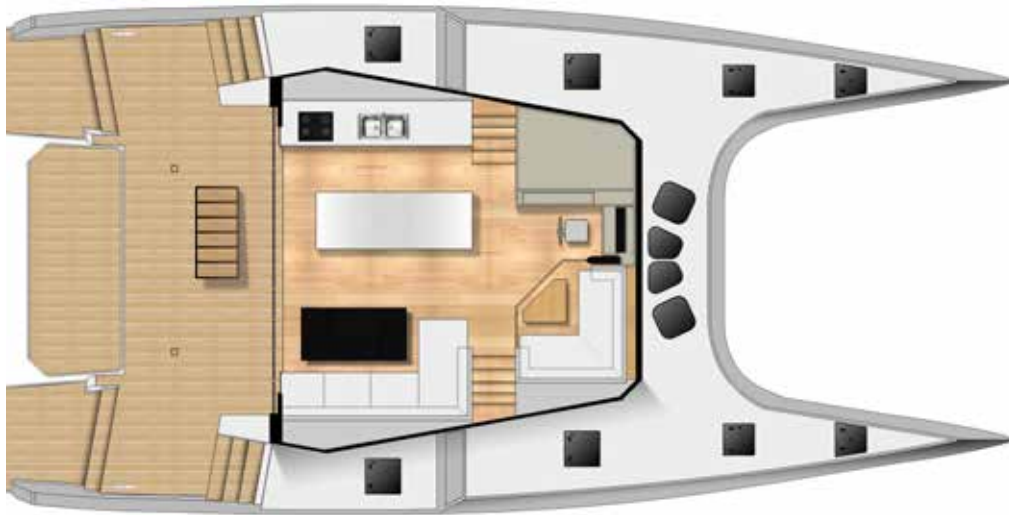
3 CABIN LAYOUT
