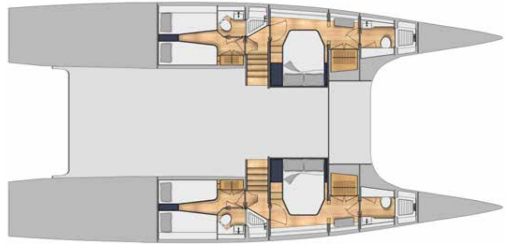
4 CABIN LAYOUT
